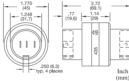
MER90009 Terminal 16-14 AWG
