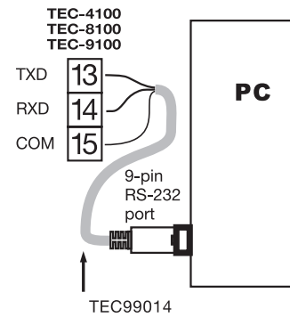
Figure 2.22 RS-232 Wiring
