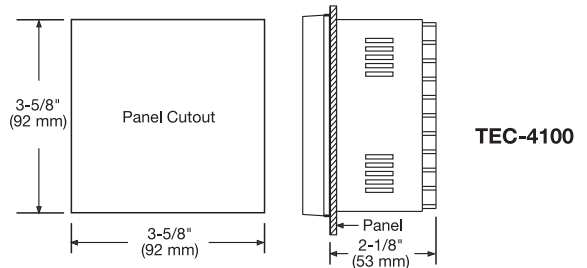
Figure 2.1 Mounting Dimensions
