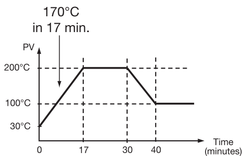
Figure 3.5 RAMP Function
